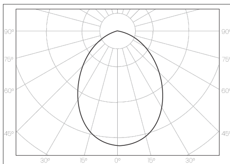
polar curve
